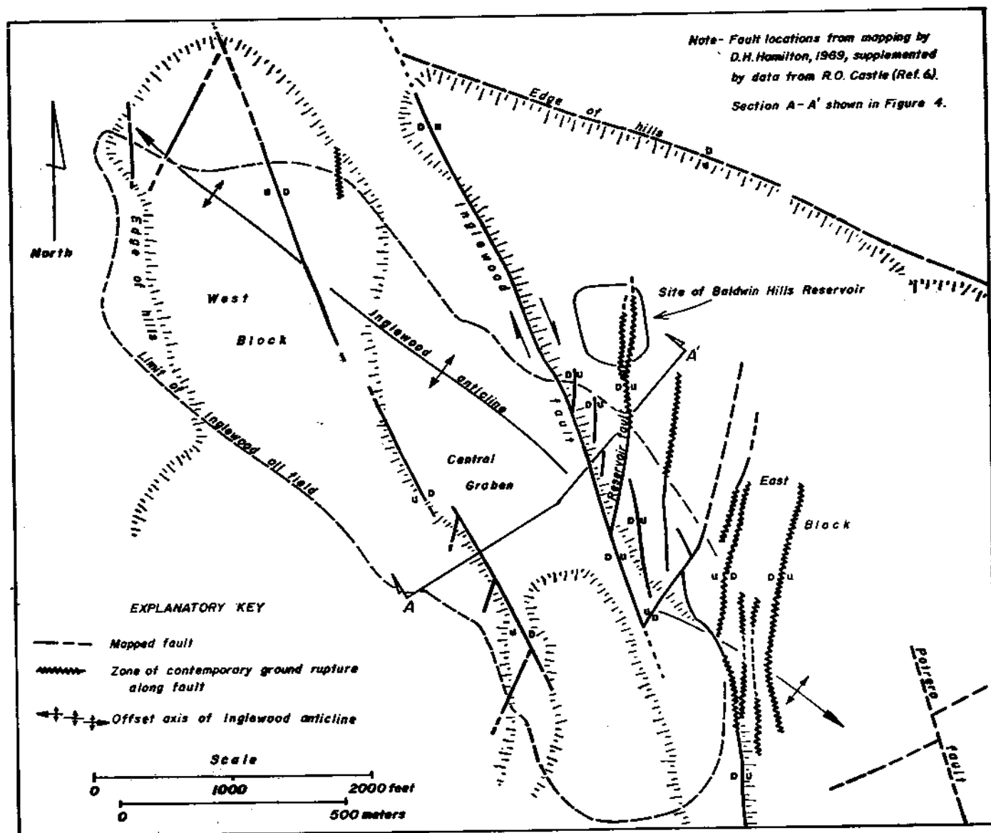
Fig. 3. Geologic map of the Baldwin Hills.
