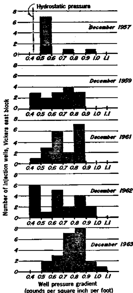
Fig. 5. Injection history for Vickers east block, 1957-63.
